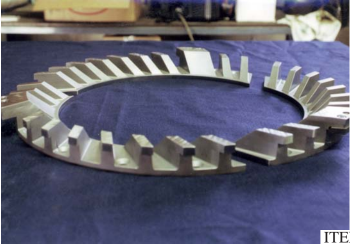
SHREDDER ROTOR MANUFACTURED AS TRI-SEGMENTAL SYSTEM; SHOWN WITH CUTTER SET
