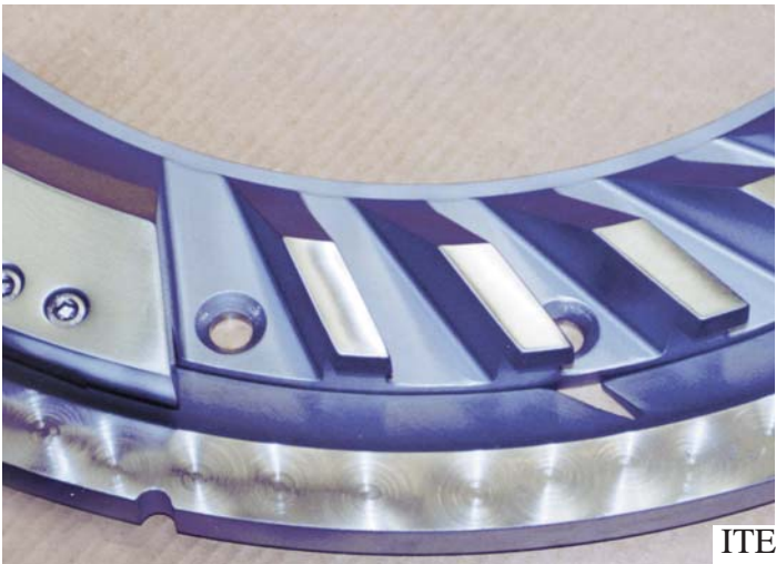
CLOSE UP AND OVERVIEW OF NEW ROTOR AND ANVIL
